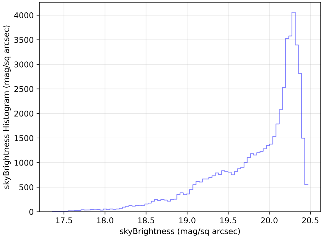
too_elab_r32_d3_gz_v3.4_10yrs Yr 1 i band: skyBrightness Histogram
