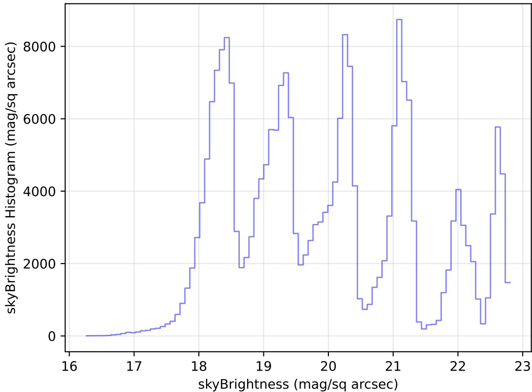
too_elab_r32_d3_gz_v3.4_10yrs Yr 1 all bands: skyBrightness Histogram
