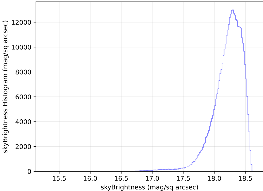
too_elab_r32_d3_gz_v3.4_10yrs WFD y band: skyBrightness Histogram
