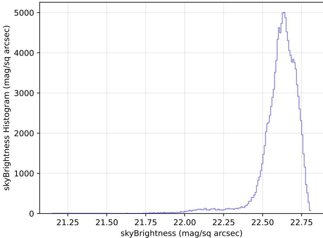
too_elab_r32_d3_gz_v3.4_10yrs WFD u band: skyBrightness Histogram
