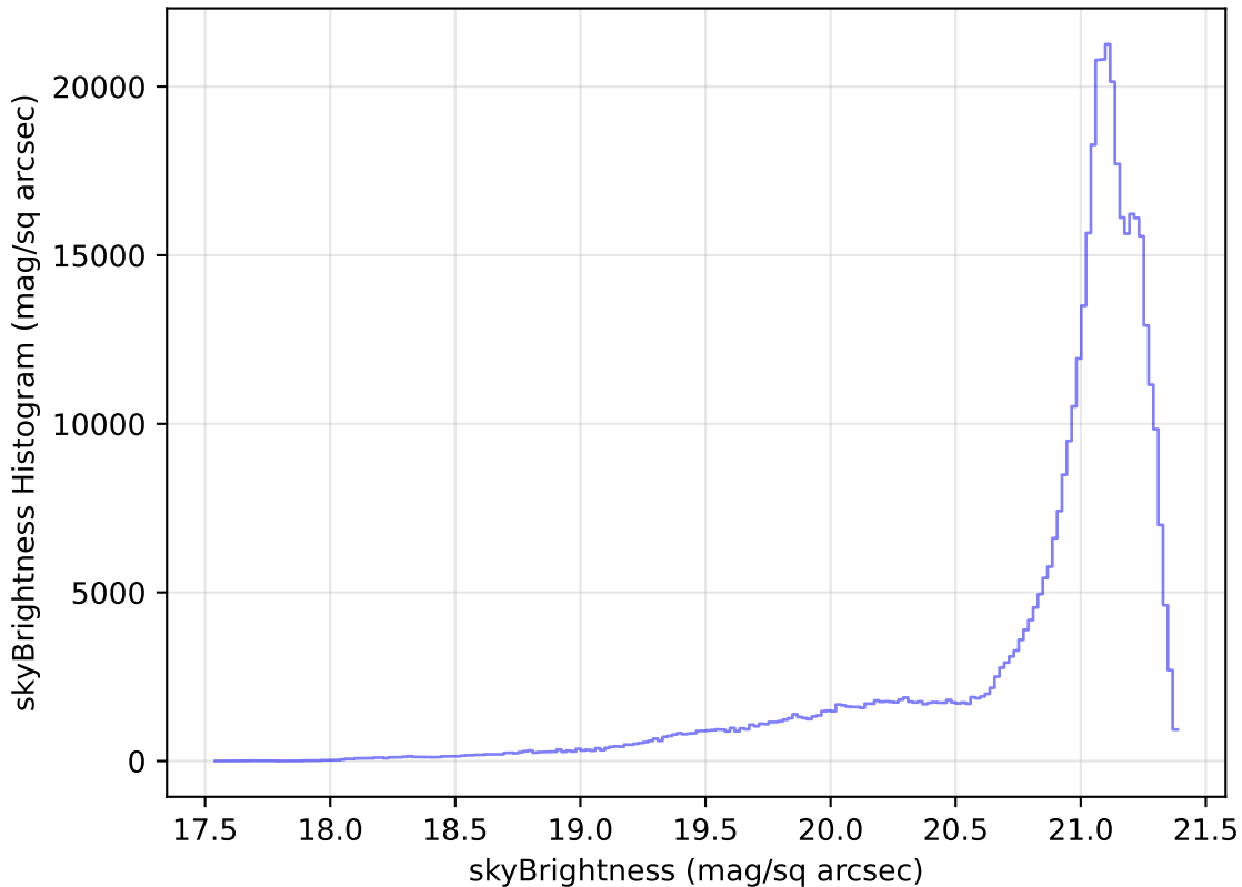
too_elab_r32_d3_gz_v3.4_10yrs WFD r band: skyBrightness Histogram
