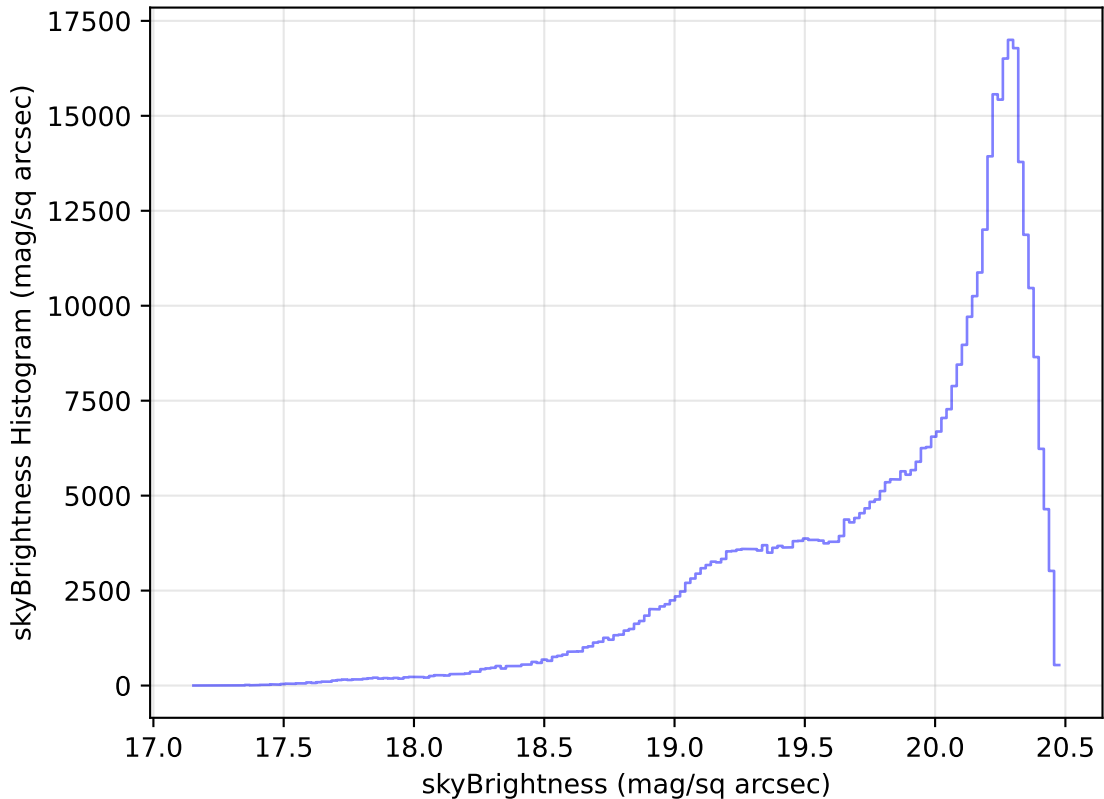
too_elab_r32_d3_gz_v3.4_10yrs WFD i band: skyBrightness Histogram
