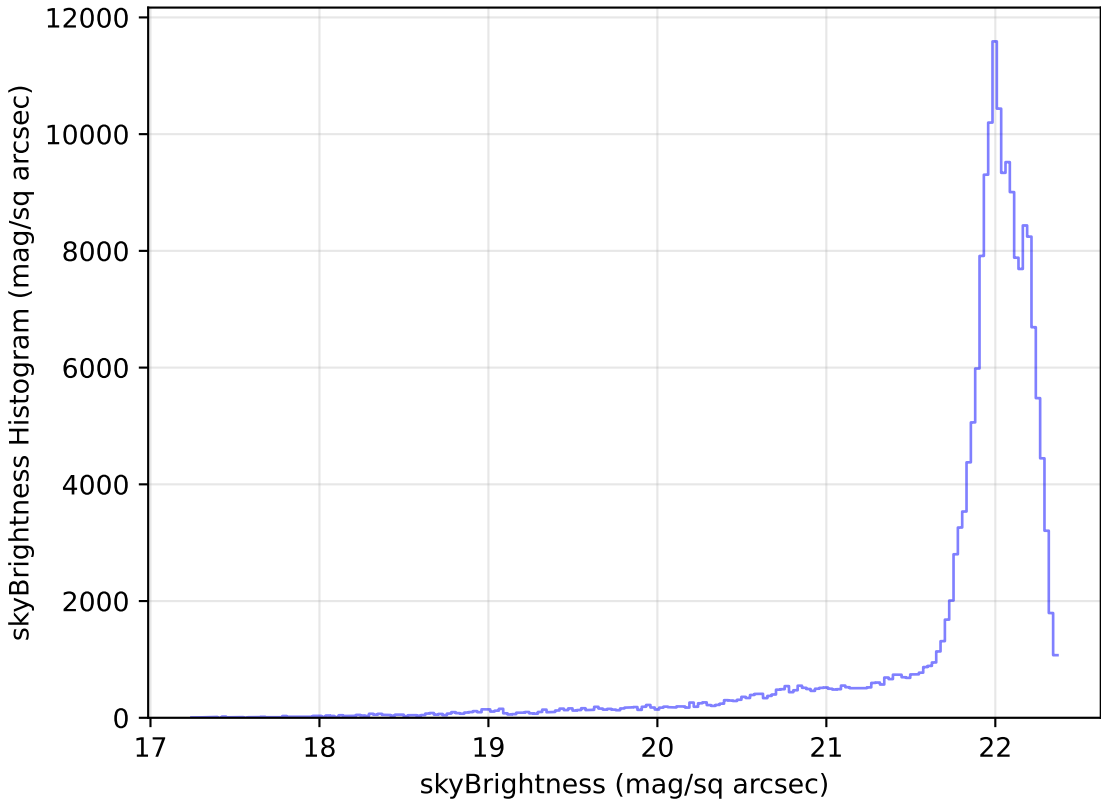
too_elab_r32_d3_gz_v3.4_10yrs WFD g band: skyBrightness Histogram
