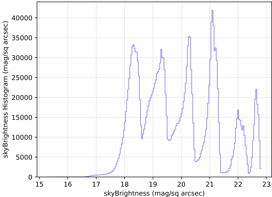
too_elab_r32_d3_gz_v3.4_10yrs WFD all bands: skyBrightness Histogram
