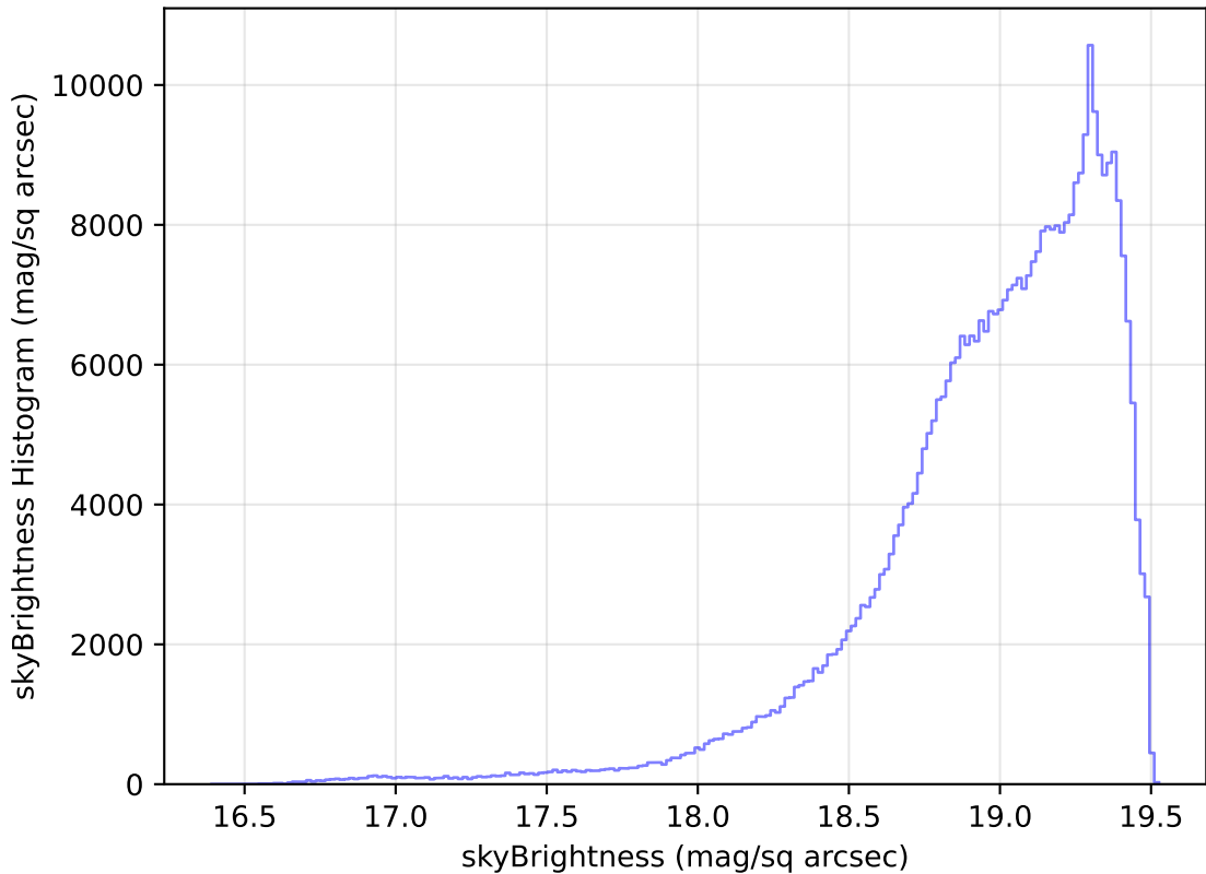
too_elab_r32_d3_gz_v3.4_10yrs All sky z band: skyBrightness Histogram
