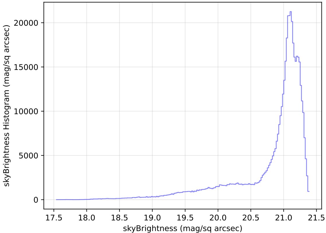
too_elab_r32_d3_gz_v3.4_10yrs All sky r band: skyBrightness Histogram
