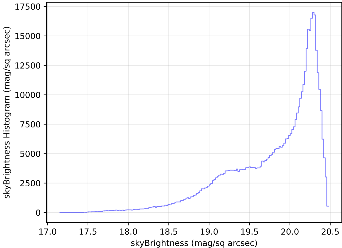
too_elab_r32_d3_gz_v3.4_10yrs All sky i band: skyBrightness Histogram
