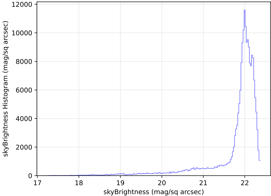
too_elab_r32_d3_gz_v3.4_10yrs All sky g band: skyBrightness Histogram
