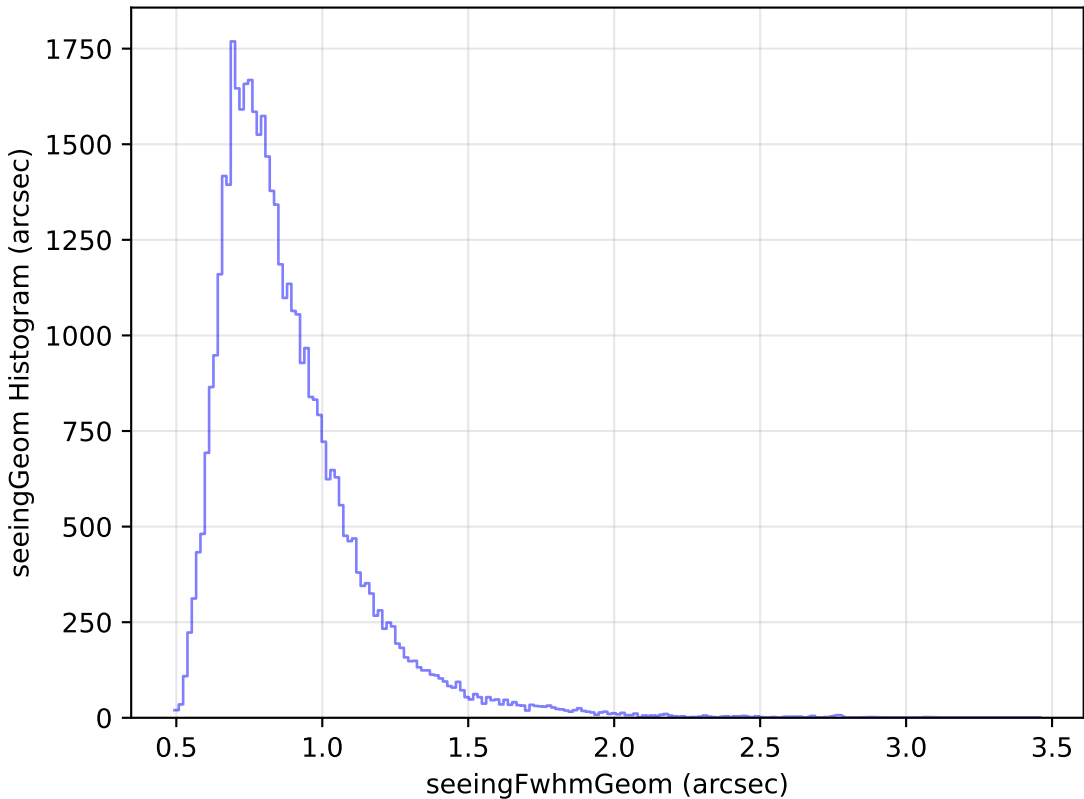
too_elab_r32_d3_gz_v3.4_10yrs Yr 1 z band: seeingGeom Histogram
