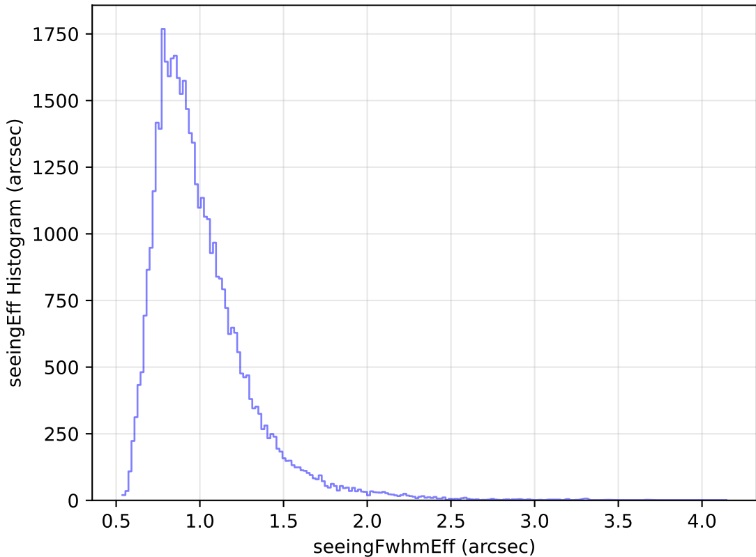
too_elab_r32_d3_gz_v3.4_10yrs Yr 1 z band: seeingEff Histogram
