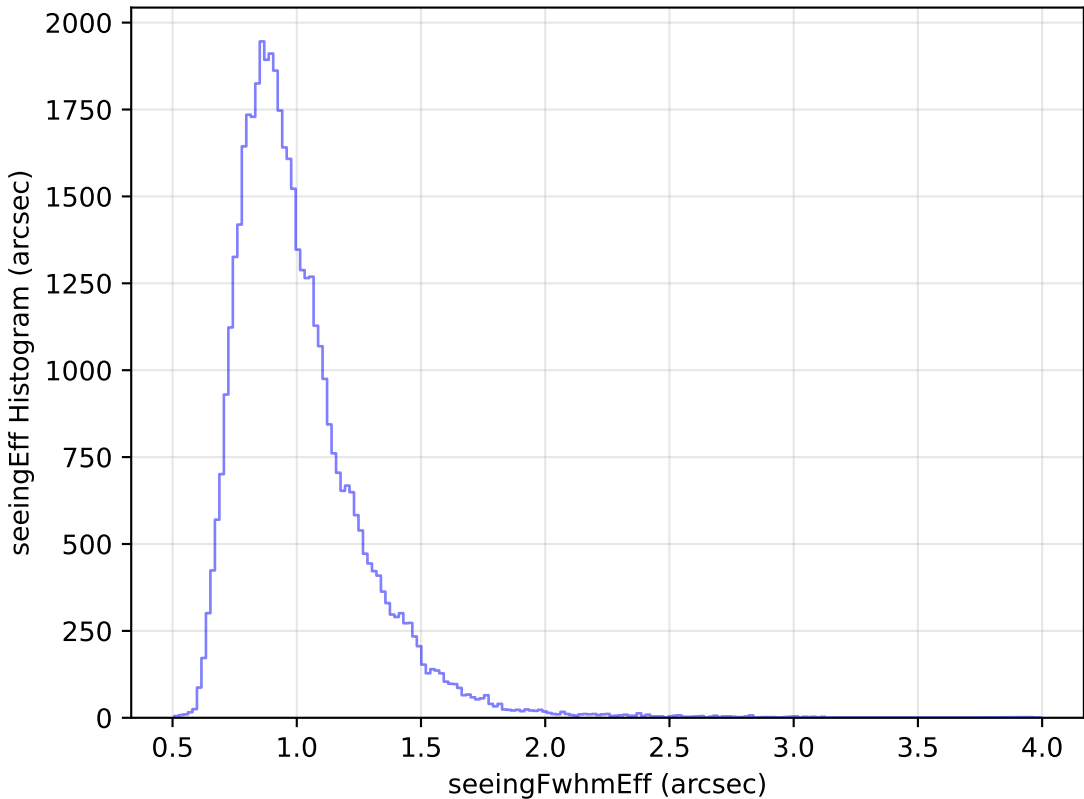
too_elab_r32_d3_gz_v3.4_10yrs Yr 1 y band: seeingEff Histogram
