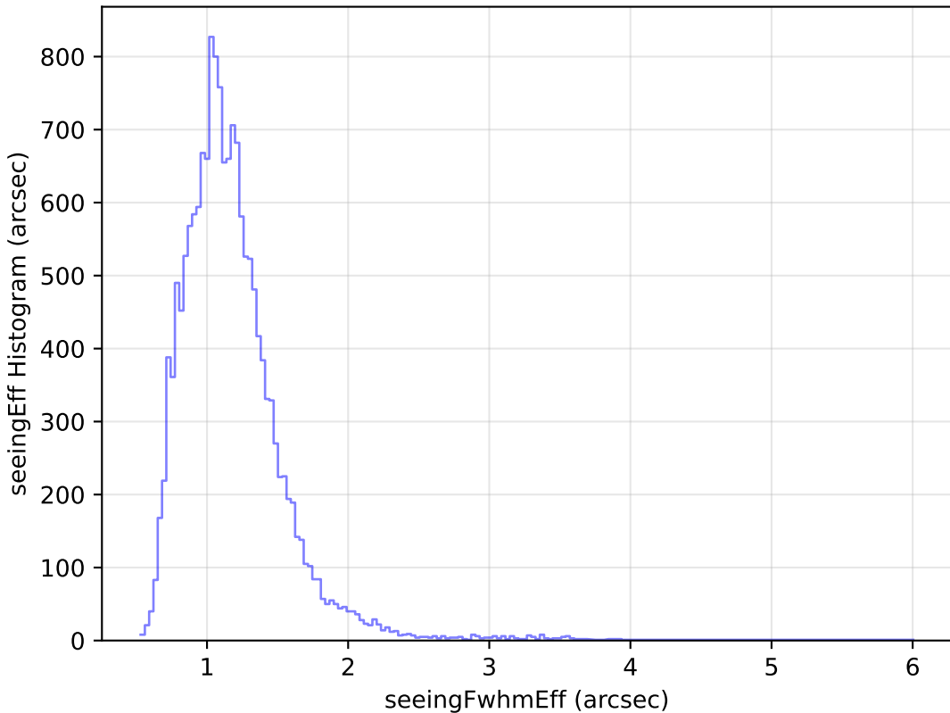
too_elab_r32_d3_gz_v3.4_10yrs Yr 1 u band: seeingEff Histogram
