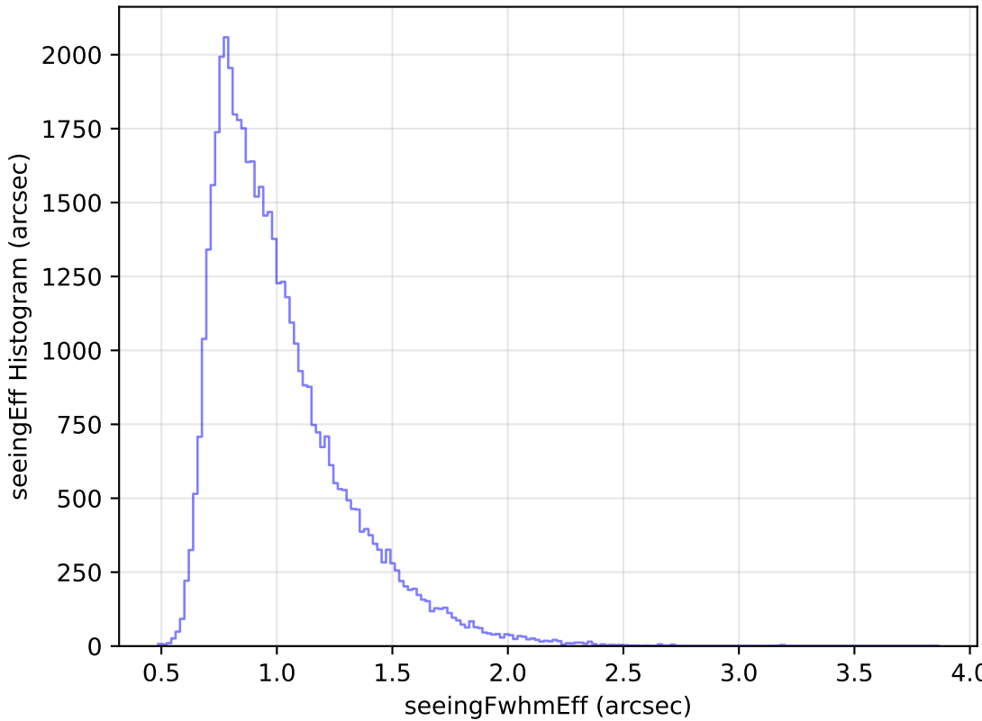
too_elab_r32_d3_gz_v3.4_10yrs Yr 1 r band: seeingEff Histogram
