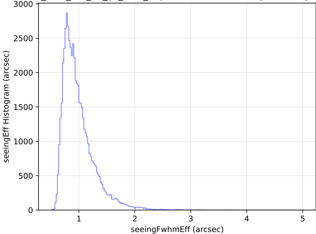
too_elab_r32_d3_gz_v3.4_10yrs Yr 1 i band: seeingEff Histogram
