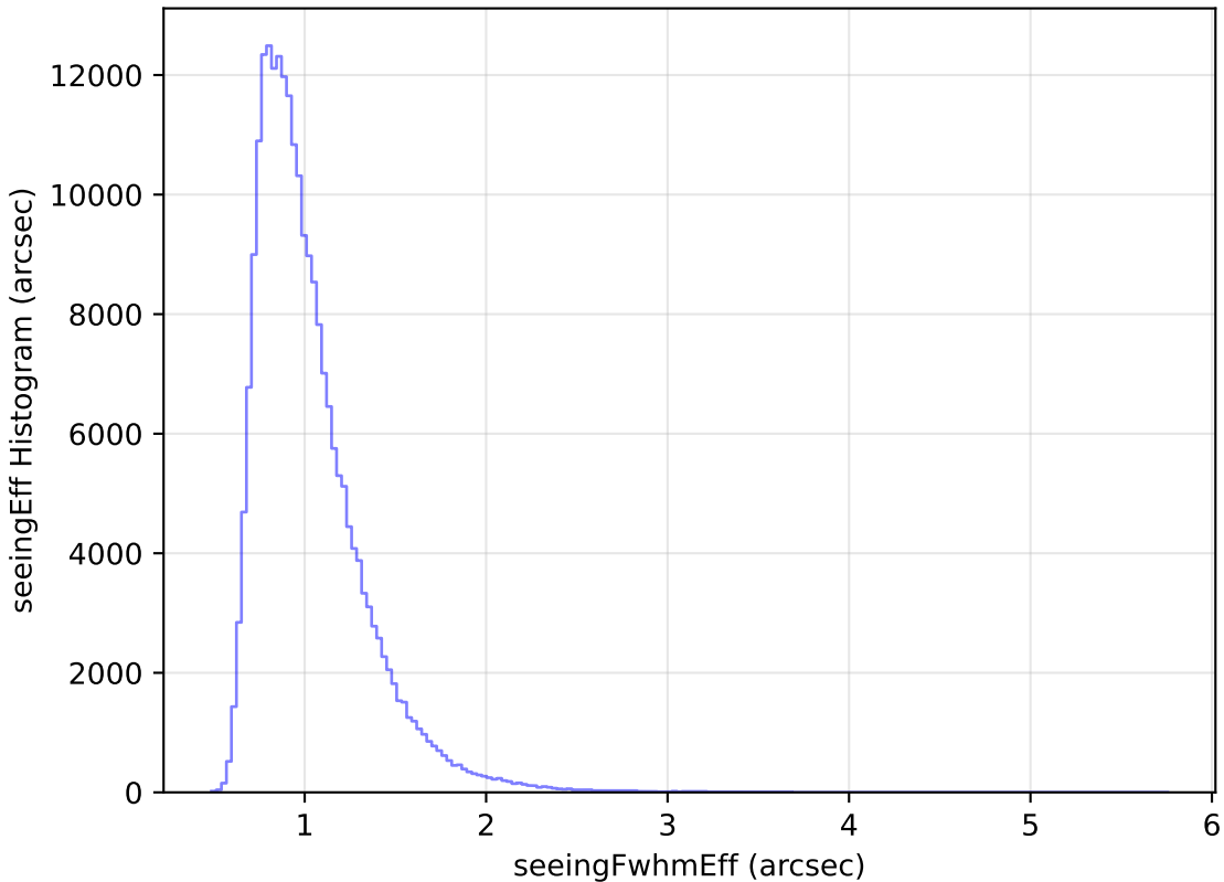
too_elab_r32_d3_gz_v3.4_10yrs Yr 1 all bands: seeingEff Histogram
