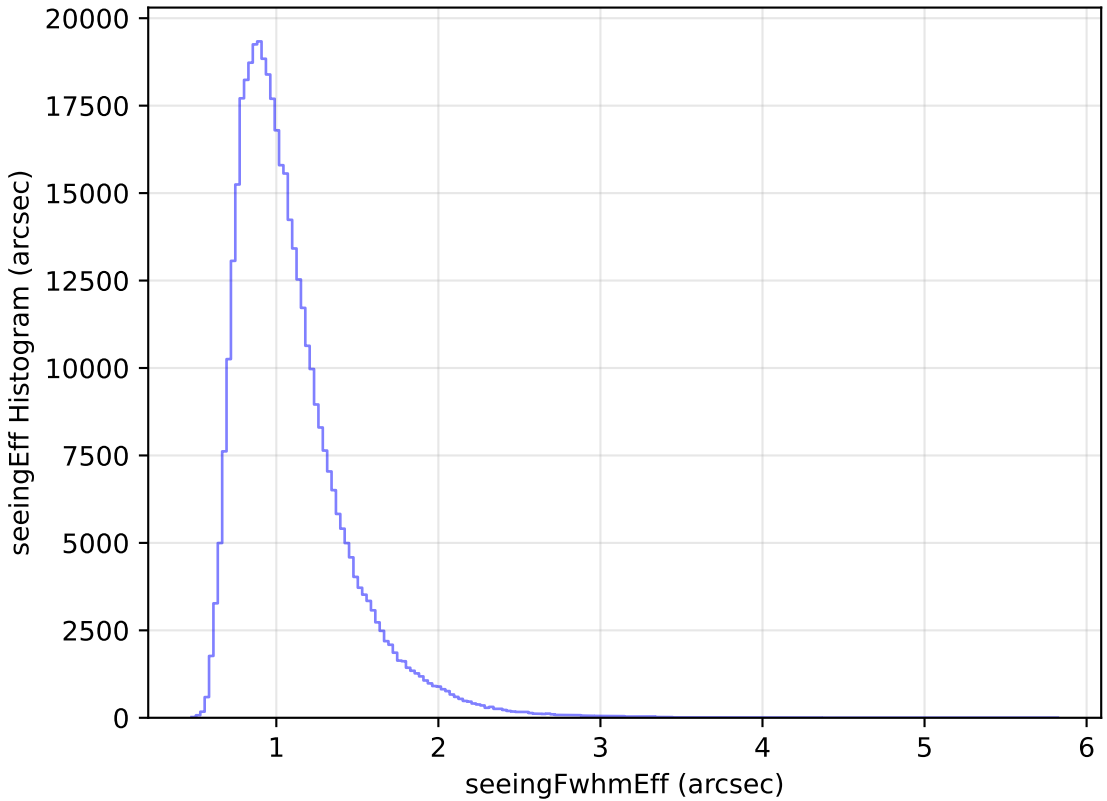
too_elab_r32_d3_gz_v3.4_10yrs WFD z band: seeingEff Histogram
