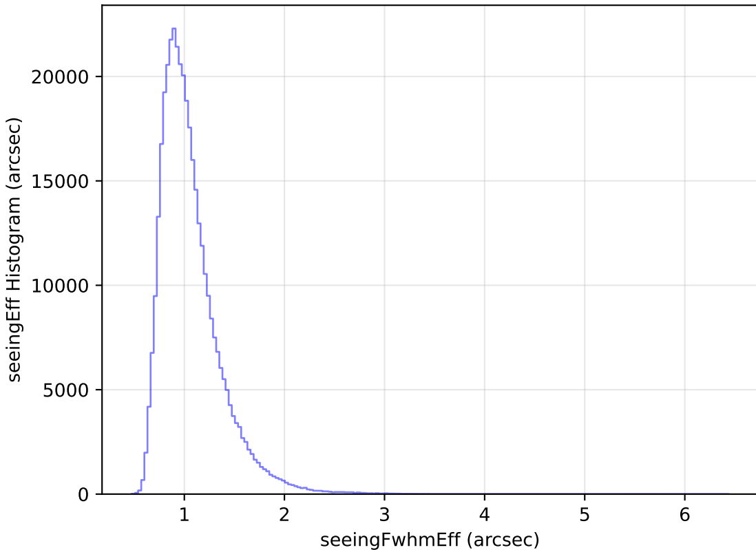
too_elab_r32_d3_gz_v3.4_10yrs WFD y band: seeingEff Histogram
