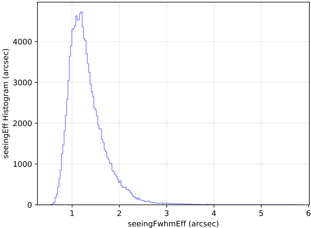
too_elab_r32_d3_gz_v3.4_10yrs WFD u band: seeingEff Histogram
