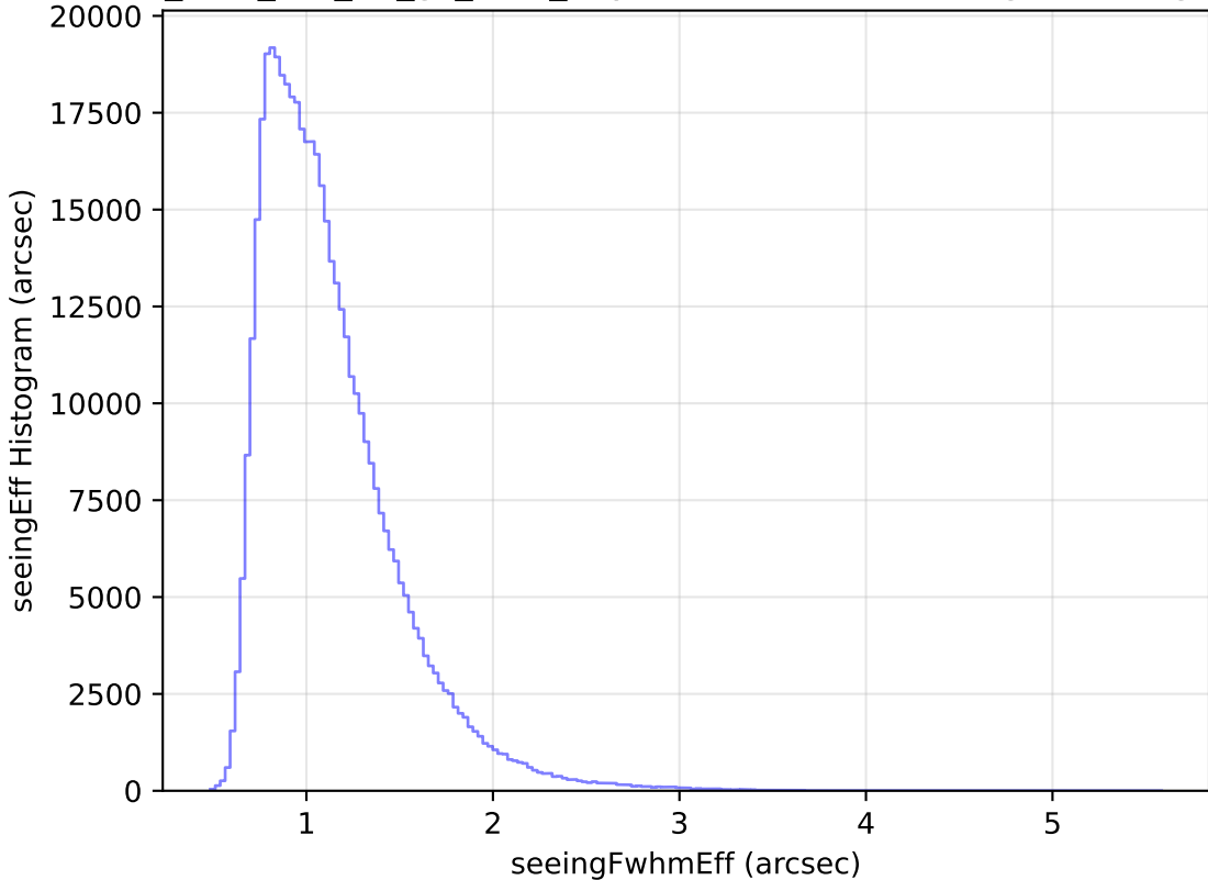
too_elab_r32_d3_gz_v3.4_10yrs WFD r band: seeingEff Histogram
