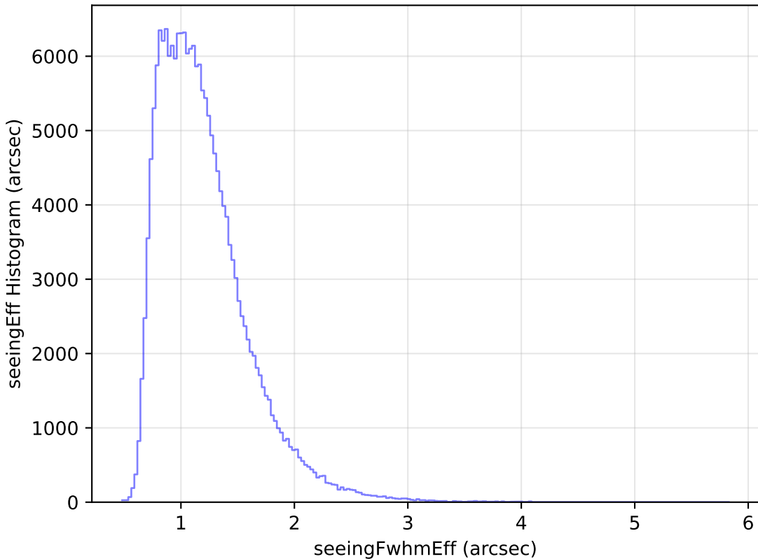
too_elab_r32_d3_gz_v3.4_10yrs WFD g band: seeingEff Histogram
