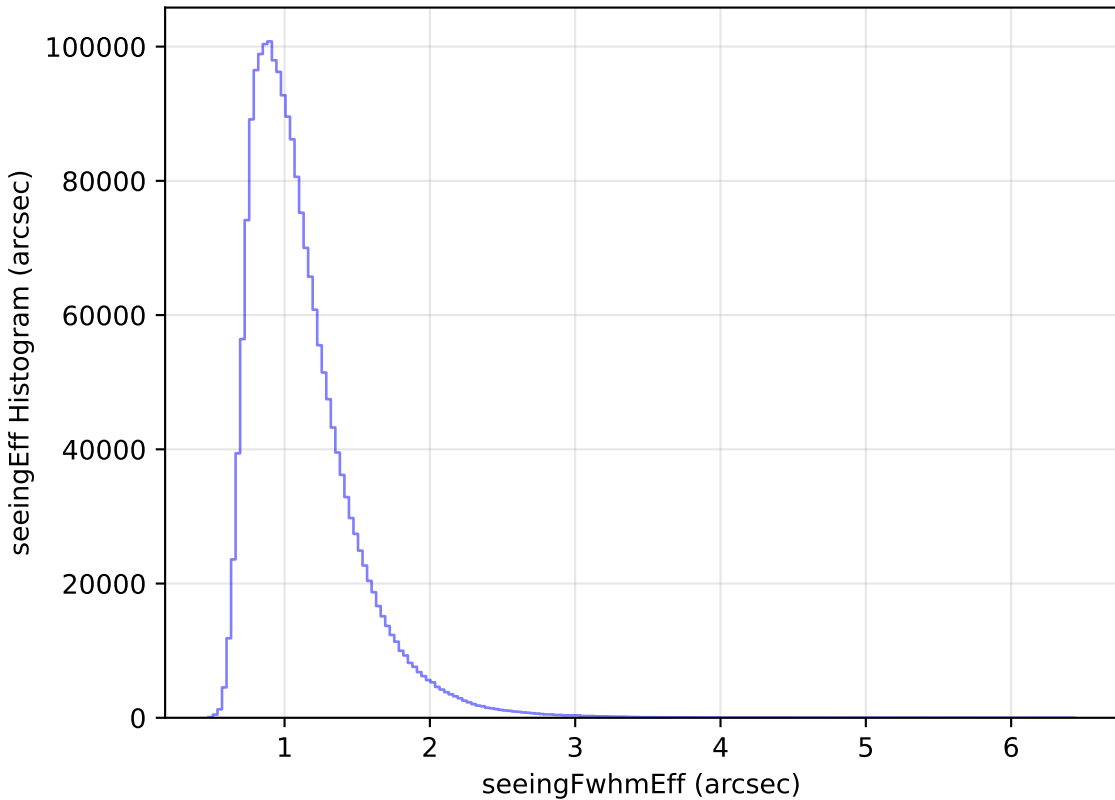
too_elab_r32_d3_gz_v3.4_10yrs WFD all bands: seeingEff Histogram
