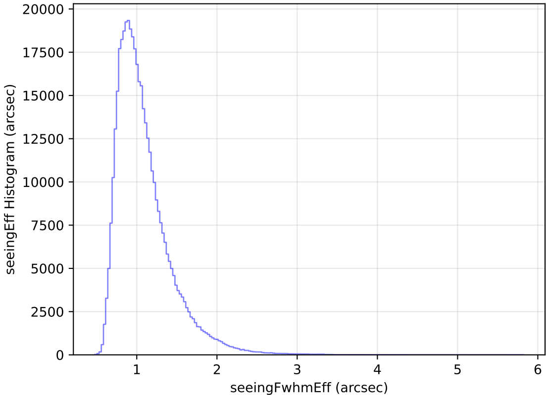
too_elab_r32_d3_gz_v3.4_10yrs All sky z band: seeingEff Histogram
