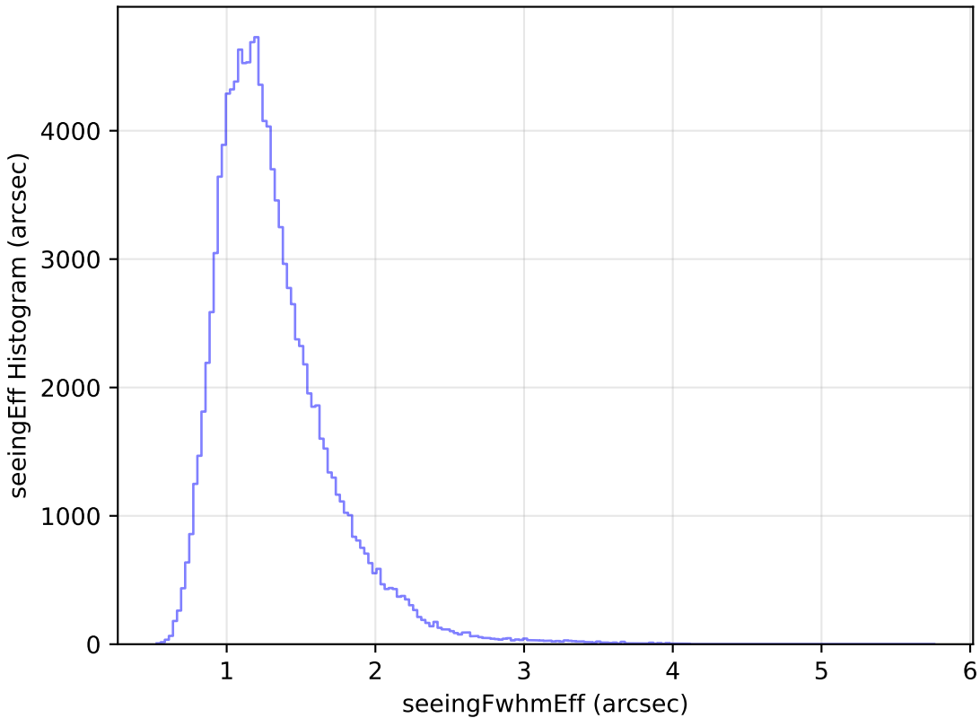
too_elab_r32_d3_gz_v3.4_10yrs All sky u band: seeingEff Histogram
