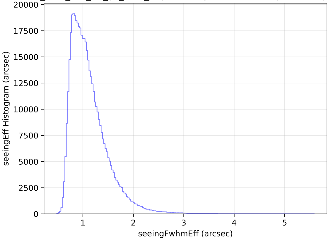
too_elab_r32_d3_gz_v3.4_10yrs All sky r band: seeingEff Histogram
