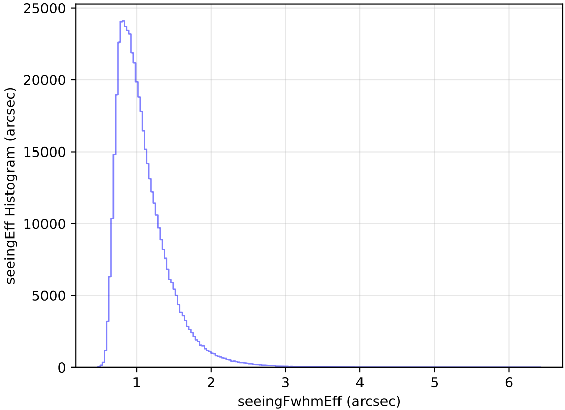
too_elab_r32_d3_gz_v3.4_10yrs All sky i band: seeingEff Histogram
