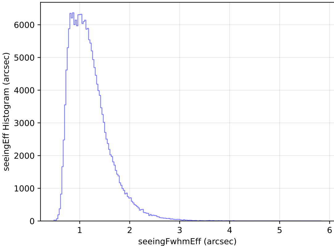
too_elab_r32_d3_gz_v3.4_10yrs All sky g band: seeingEff Histogram
