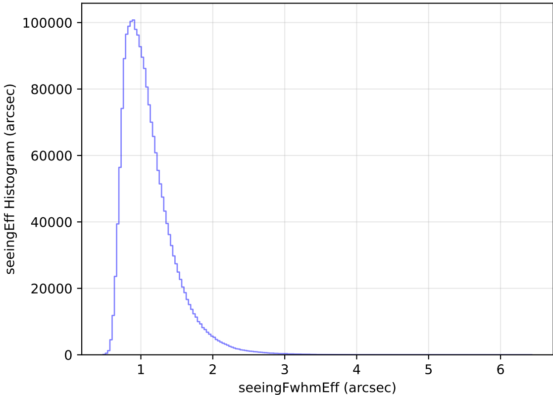
too_elab_r32_d3_gz_v3.4_10yrs All sky all bands: seeingEff Histogram
