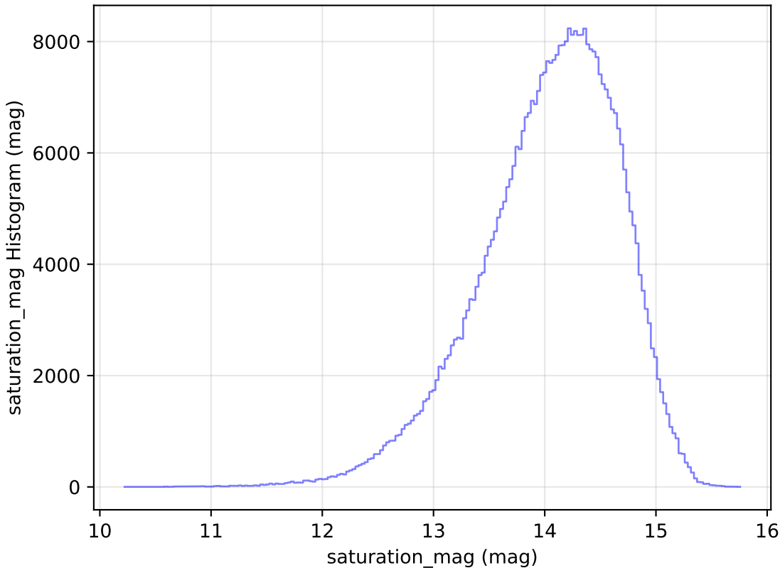
too_elab_r32_d3_gz_v3.4_10yrs WFD z band: saturation_mag Histogram
