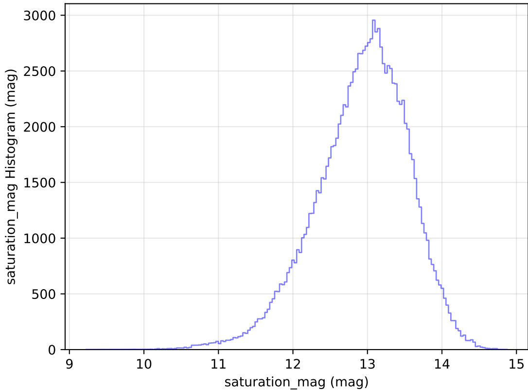
too_elab_r32_d3_gz_v3.4_10yrs WFD u band: saturation_mag Histogram
