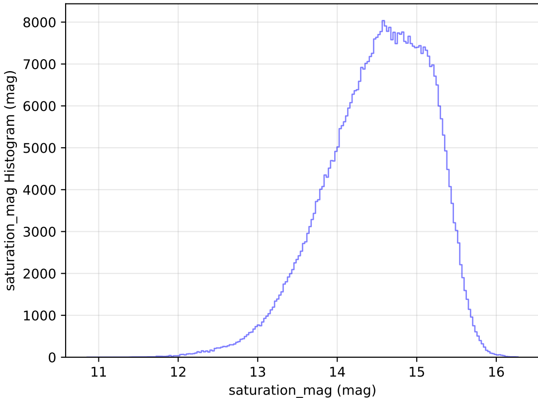
too_elab_r32_d3_gz_v3.4_10yrs WFD r band: saturation_mag Histogram
