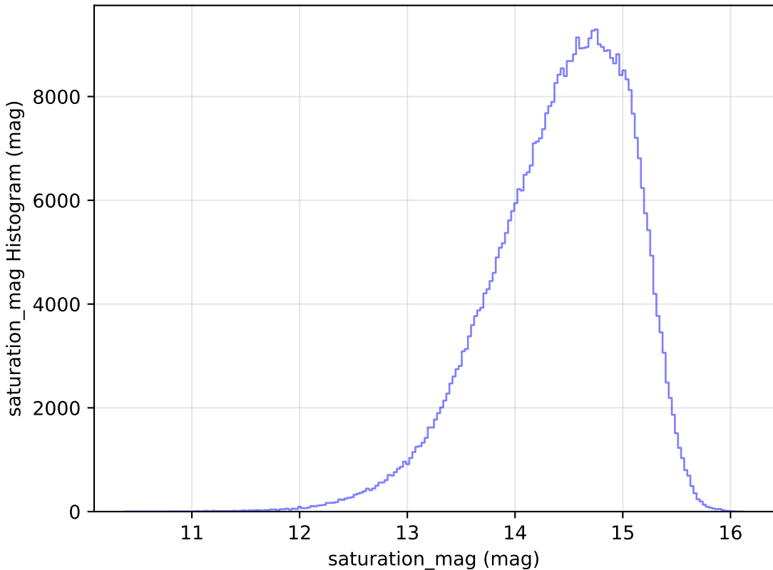
too_elab_r32_d3_gz_v3.4_10yrs WFD i band: saturation_mag Histogram
