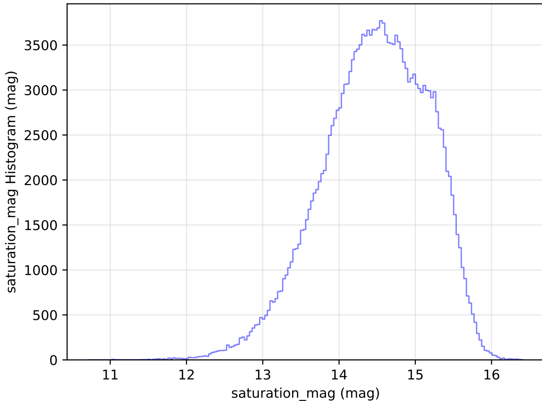
too_elab_r32_d3_gz_v3.4_10yrs WFD g band: saturation_mag Histogram
