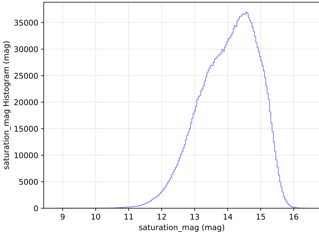
too_elab_r32_d3_gz_v3.4_10yrs WFD all bands: saturation_mag Histogram
