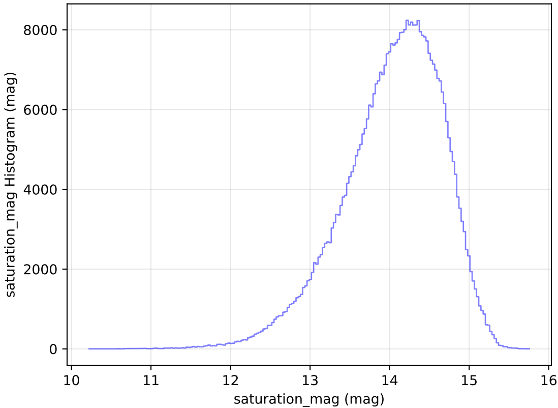
too_elab_r32_d3_gz_v3.4_10yrs All sky z band: saturation_mag Histogram
