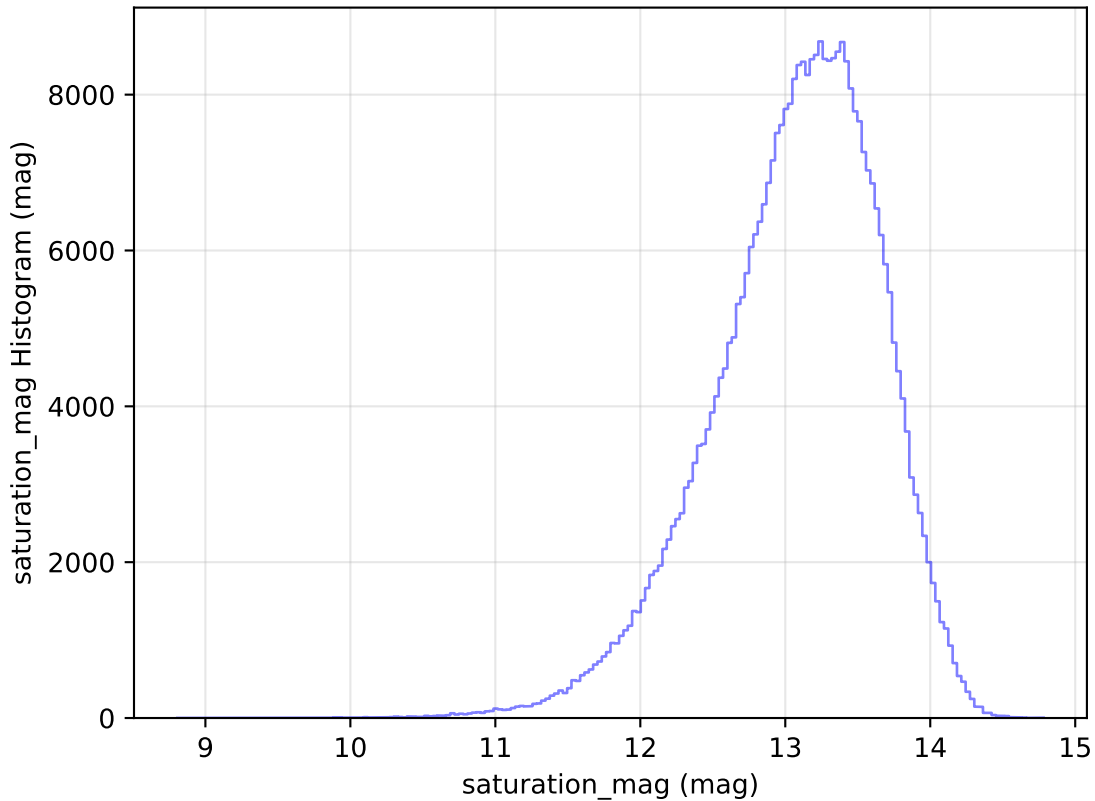
too_elab_r32_d3_gz_v3.4_10yrs All sky y band: saturation_mag Histogram
