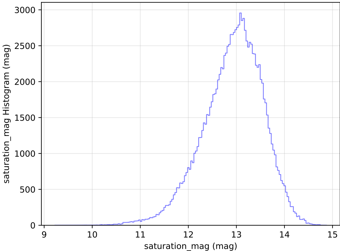
too_elab_r32_d3_gz_v3.4_10yrs All sky u band: saturation_mag Histogram
