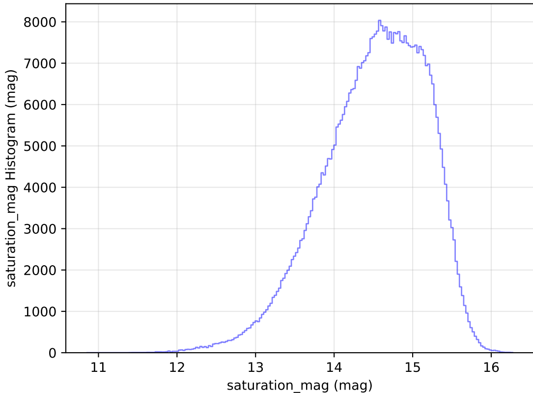
too_elab_r32_d3_gz_v3.4_10yrs All sky r band: saturation_mag Histogram
