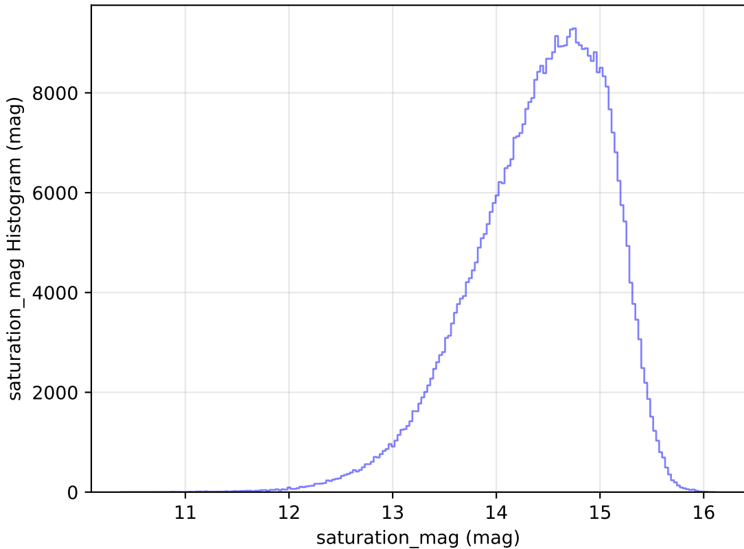
too_elab_r32_d3_gz_v3.4_10yrs All sky i band: saturation_mag Histogram
