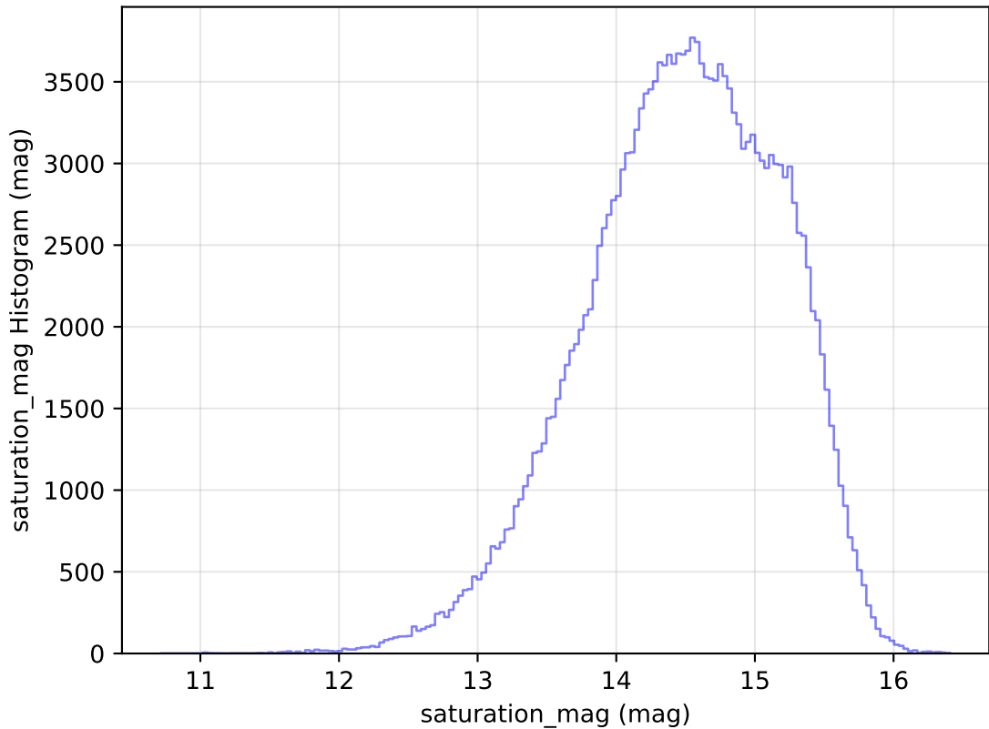
too_elab_r32_d3_gz_v3.4_10yrs All sky g band: saturation_mag Histogram
