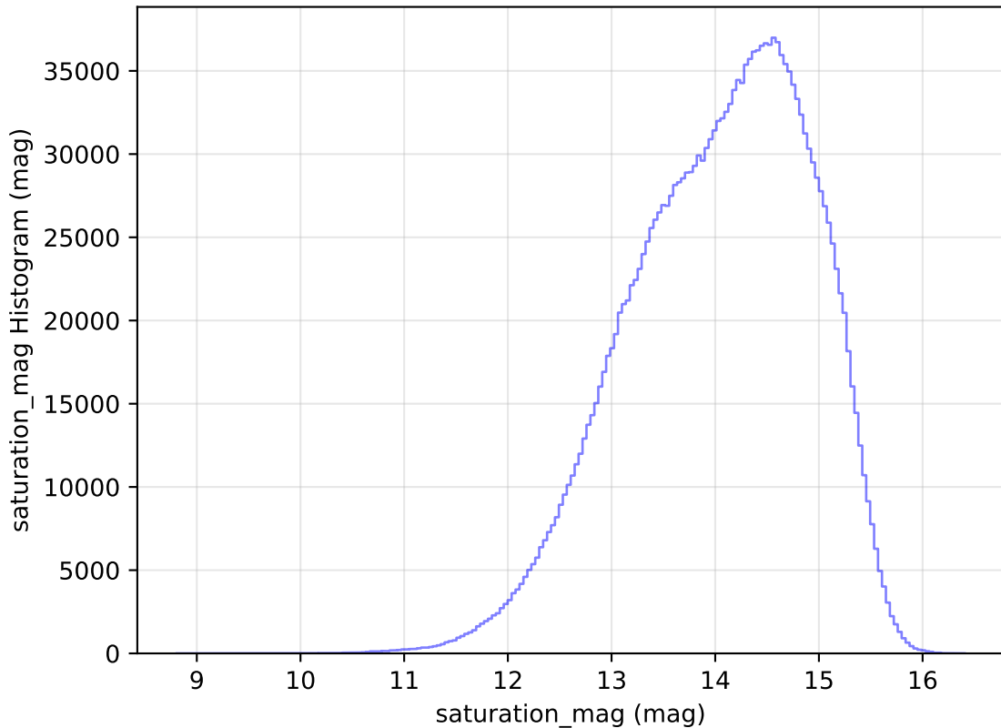
too_elab_r32_d3_gz_v3.4_10yrs All sky all bands: saturation_mag Histogram
