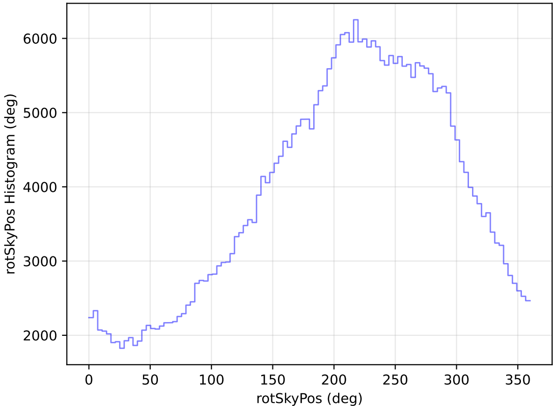
too_elab_r32_d3_gz_v3.4_10yrs WFD y band: rotSkyPos Histogram
