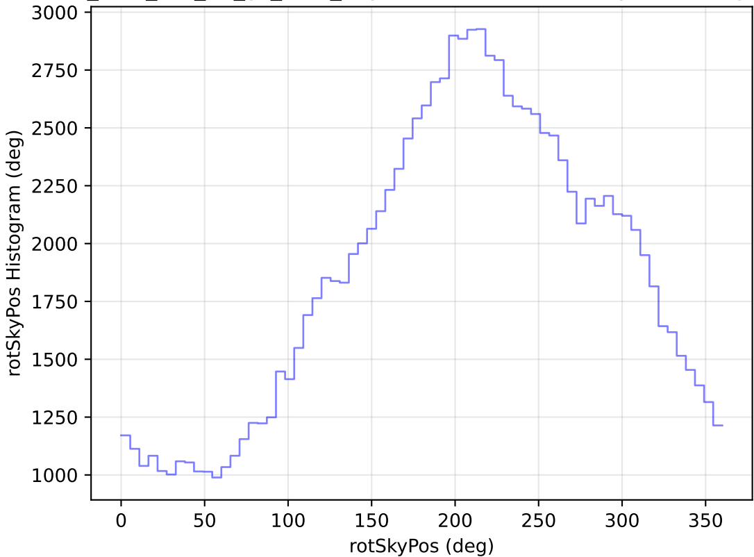
too_elab_r32_d3_gz_v3.4_10yrs WFD u band: rotSkyPos Histogram
