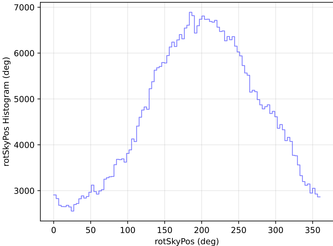
too_elab_r32_d3_gz_v3.4_10yrs WFD r band: rotSkyPos Histogram
