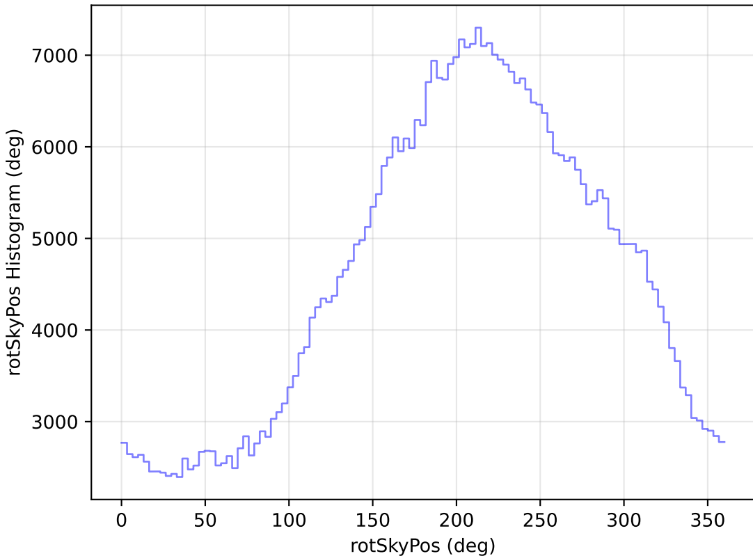
too_elab_r32_d3_gz_v3.4_10yrs WFD i band: rotSkyPos Histogram
