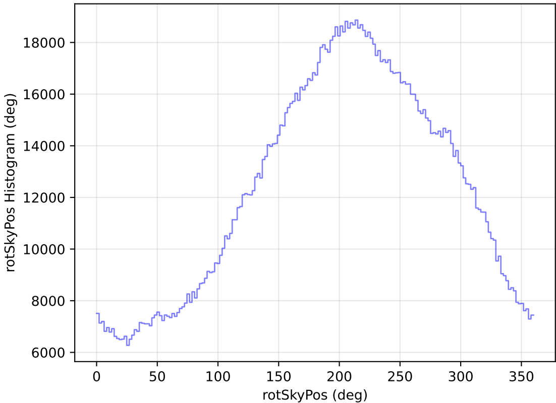
too_elab_r32_d3_gz_v3.4_10yrs WFD all bands: rotSkyPos Histogram
