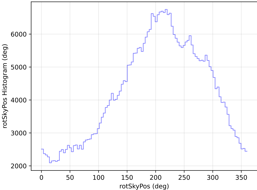
too_elab_r32_d3_gz_v3.4_10yrs All sky z band: rotSkyPos Histogram
